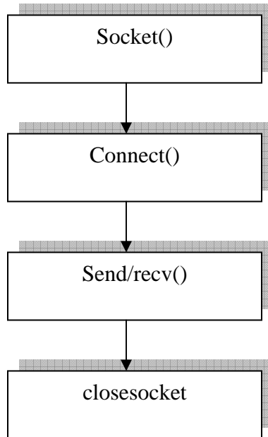
Figure 1 Client Connection
