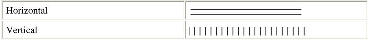
Figure 3 Brush Styles
